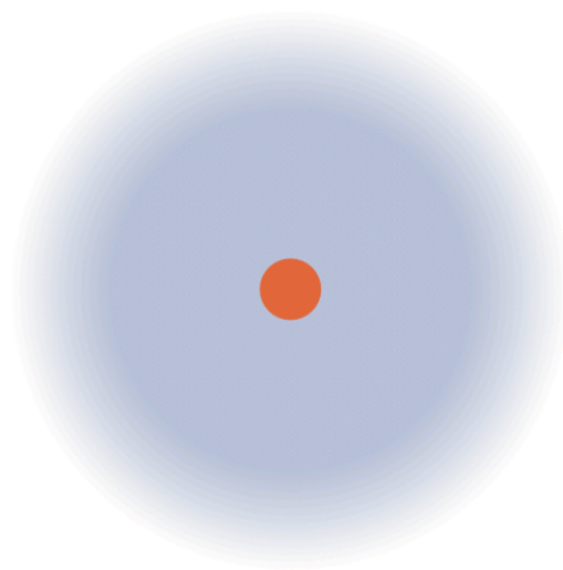
Electron Cloud Model
