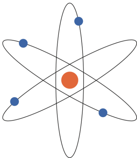
Electron Orbit Model
